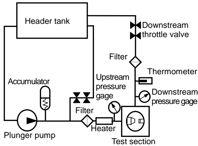
Figure 1: Cavitating jet apparatus
